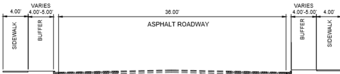
Figure 5: Freedom Way Existing Typical Section
